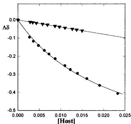
Figure 3. Titration of ACh iodide with host 1 (▼) and host 2a (●) \text{NCH}_3 protons. Points are experimental and curves are calculated
