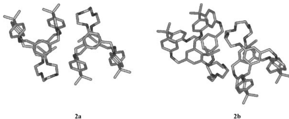
Figure 2. The dimeric packing of 2a and 2b . The dimerization of 2b is tennis ball-like whereas with 2a the cavities are exactly facing. Hydrogen atoms and n -hexane molecules are excluded for clarity
