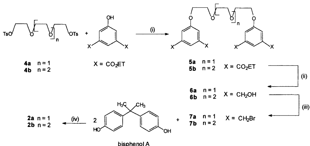
Scheme 1. Synthesis of cyclophanes 2a and 2b . (i) \text{K}_2\text{CO}_3 , \text{CH}_3\text{CN} ; (ii) \text{LiAlH}_4 , THF; (iii) \text{PBr}_3 , dioxane; (iv) \text{KOH} , DMSO, high dilution
