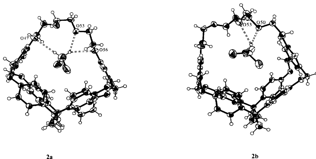
Figure 1. Molecular structures of 2a and 2b showing thermal ellipsoids at the 50% probability level. The weak hydrogen bonds of the included dichloromethane and chloroform (only the most populated orientations are shown), respectively, are shown with dotted lines
