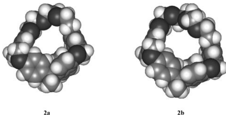
Figure 4. Van der Waals presentation of the empty cavities of 2a and 2b
